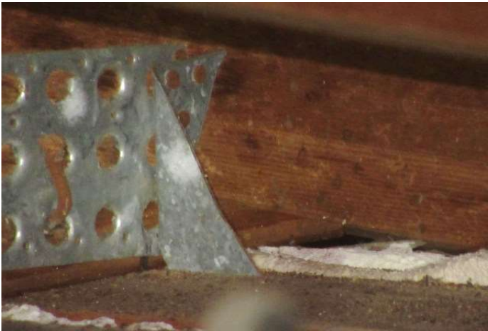
Clips with at least 3 nails into the truss
